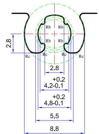
Detail 'K9' Scale 3:1
